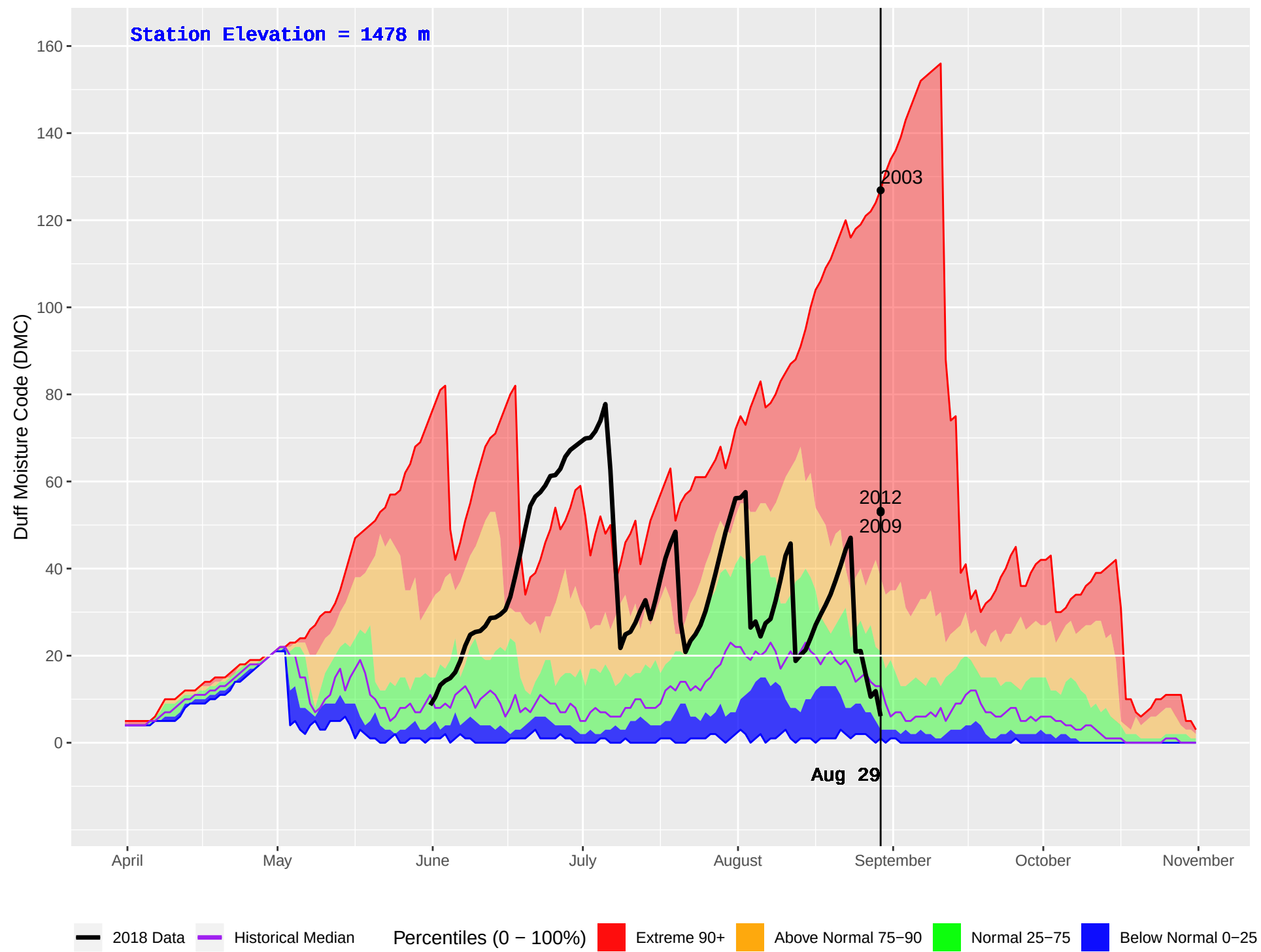
BERRY (267) : Historical (1989–2016) and Current (2018) Daily Duff Moisture Code (DMC)
