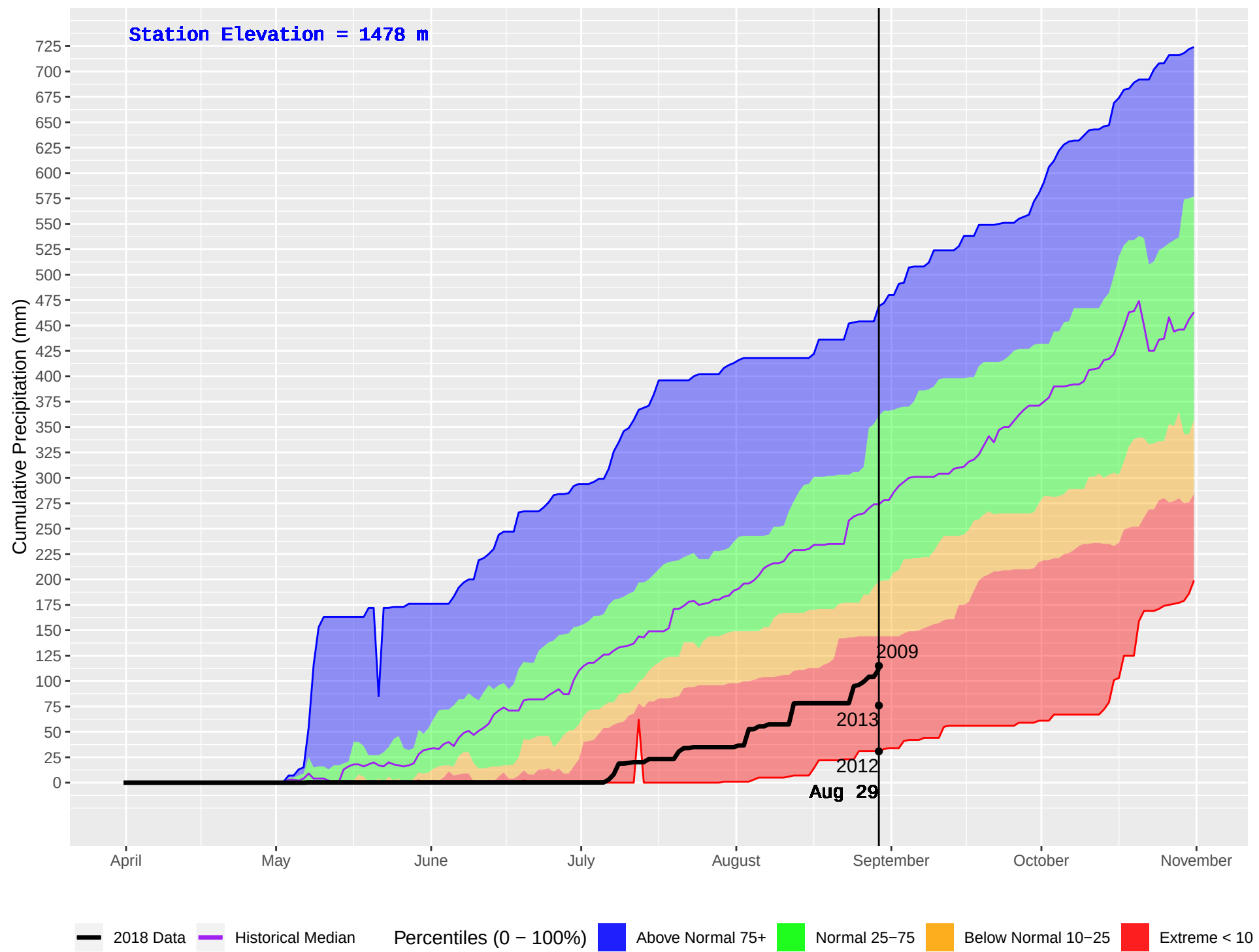
BERRY (267) : Historical (1989–2016) and Current (2018) Daily Cumulative Precipitation
