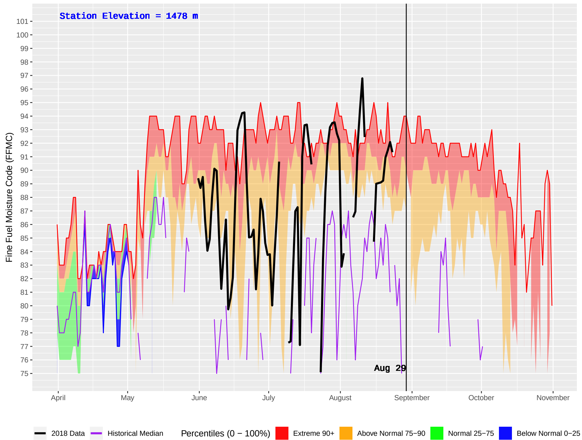
BERRY (267) : Historical (1989–2016) and Current (2018) Daily Fine Fuel Moisture Code (FFMC)
