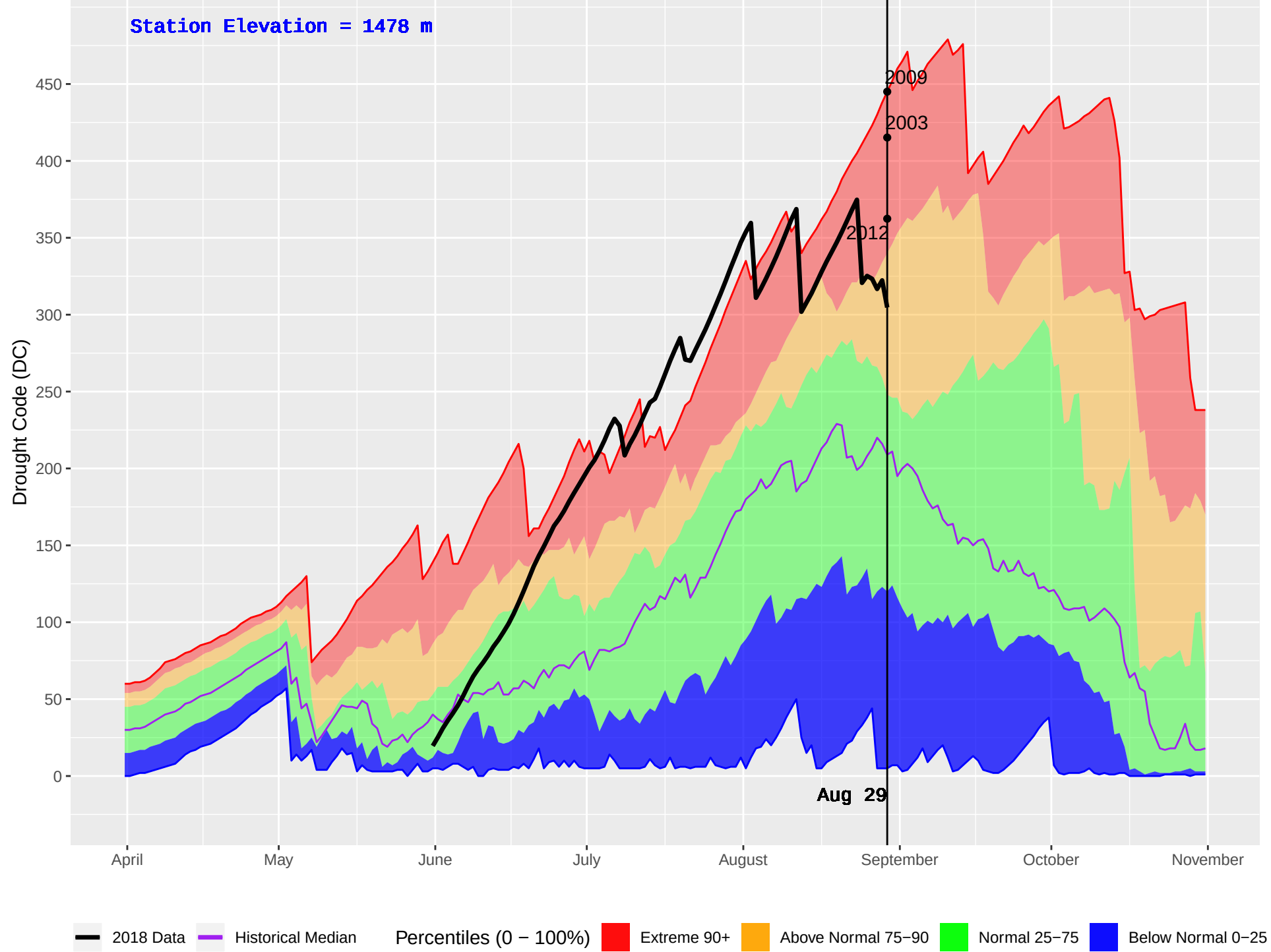
BERRY (267) : Historical (1989–2016) and Current (2018) Daily Drought Code (DC)
