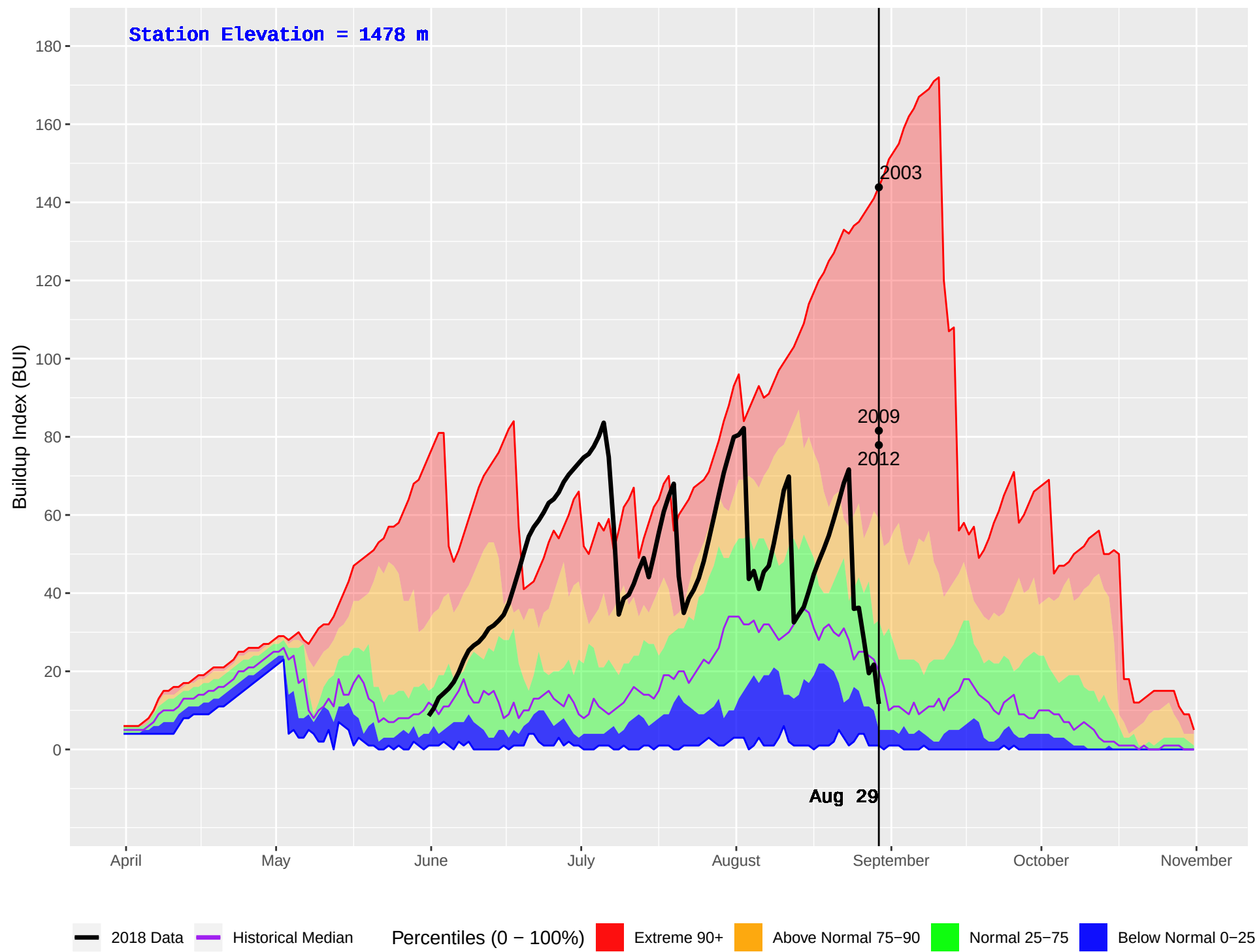
BERRY (267) : Historical (1989–2016) and Current (2018) Daily Buildup Index (BUI)
