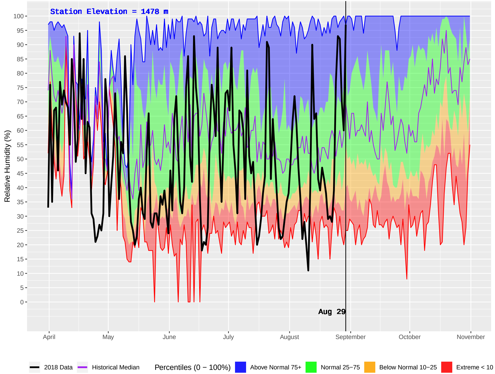
BERRY (267) : Historical (1989–2016) and Current (2018) Daily Relative Humidity
